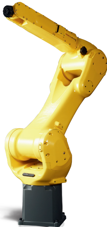
M-20iB/25 Standard model - 2 integrated solenoid valves
